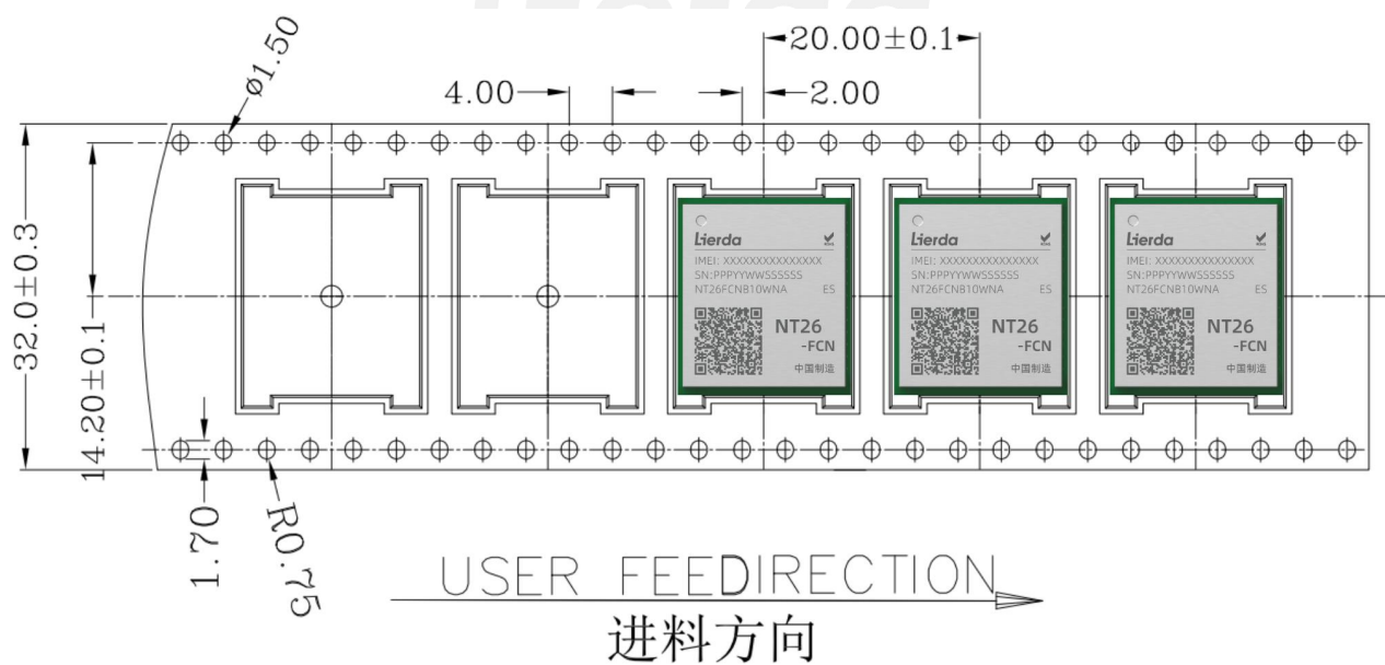
Figure 8-3 Loading Direction Indicator for Conveyor Belt
