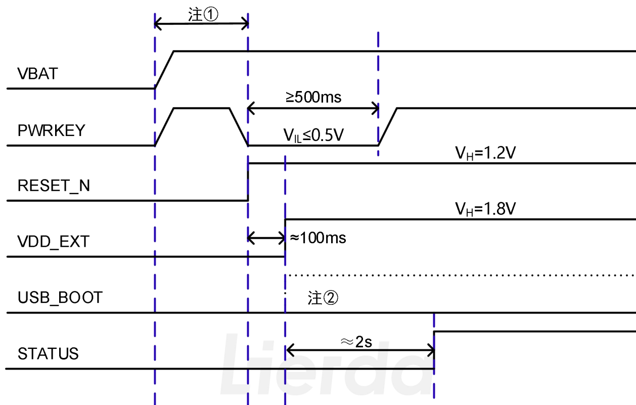
Figure 3-9 Power-On Boot Sequence Diagram
