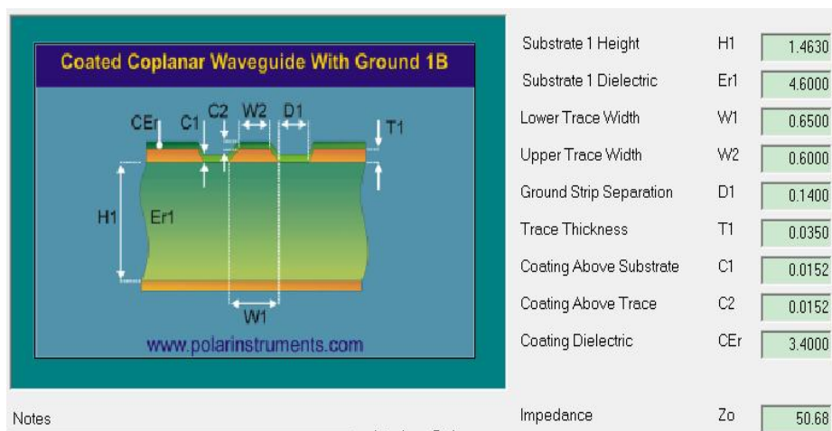
Reference for calculation of 50 ohm impedance in Figure 5-2.
