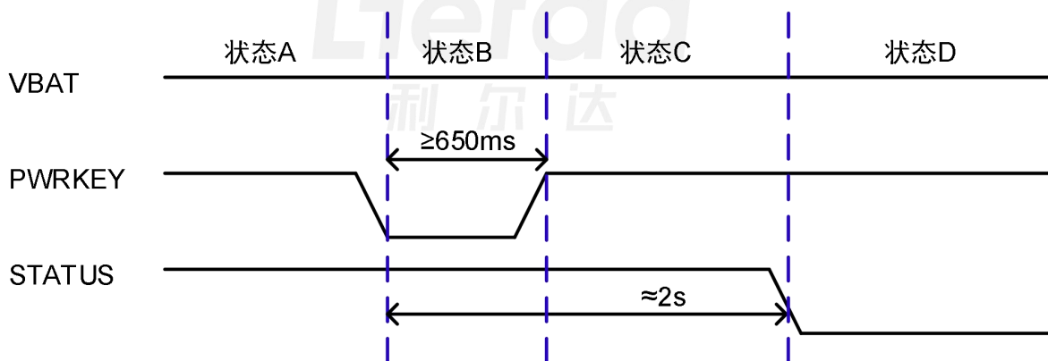
Figure 3-10 Power Key Shutdown Timing Diagram
